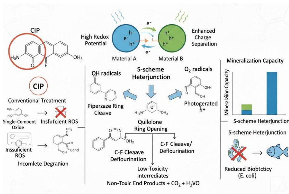
Figure 5. Schematic representation of the charge transfer mechanism in an advanced S-scheme heterojunction and the generation of reactive oxygen species (•OH, O 2 • - , h + ) leading to the cleavage and mineralization of ciprofloxacin.
